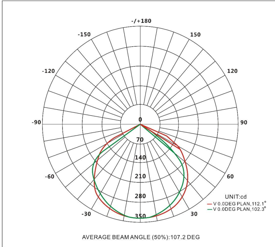
Luminous intensity distribution diagram
